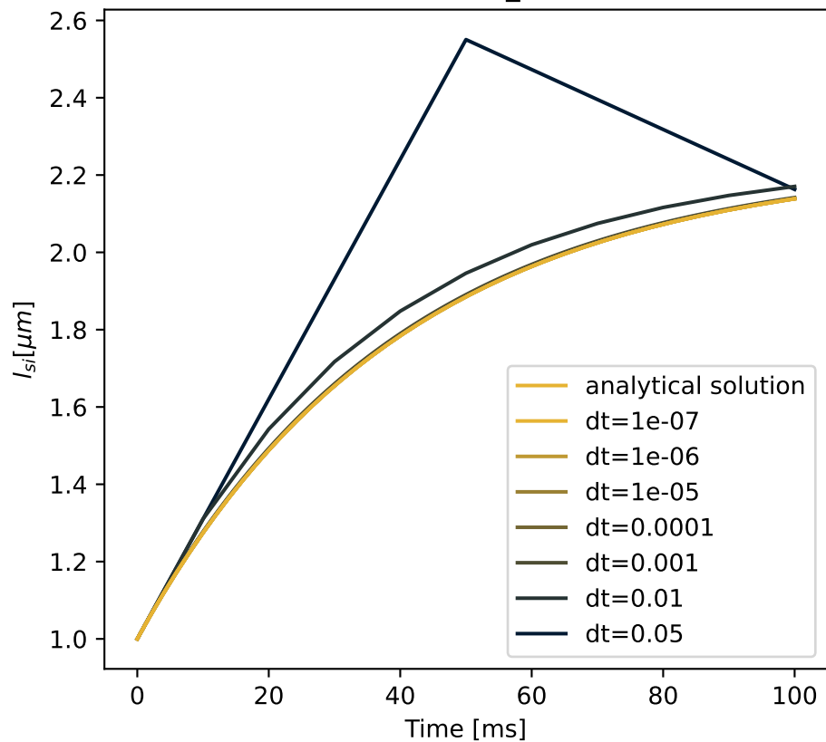
Patch2022 I si time-integrating dependency for forward_euler.
