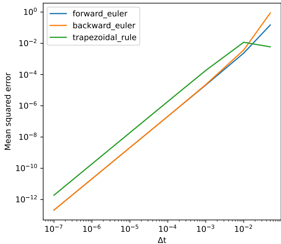
Mean squared error as function of time steps for several numerical solvers.
